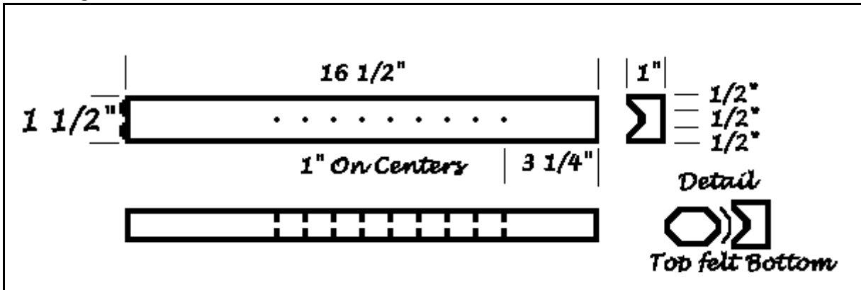
Figure 5 Lower leg dimensions
